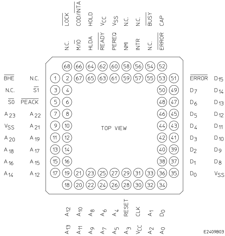
80286 68-Pin PGA Socket Diagram Top View
